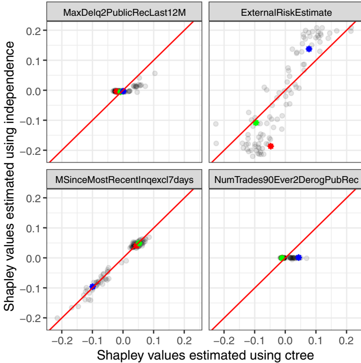
Fig. 2. The Shapley values of 100 test observations calculated using both the independence and the ctree method for four of the 23 features. (Color figure online)
